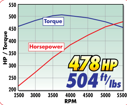
E-Force Supercharger Kit #1581 for 2004-08 F-150
