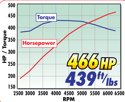
E-Force Supercharger Kit #1582 for 2010 Mustang
